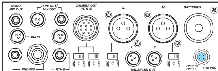
OUTPUT PANEL
