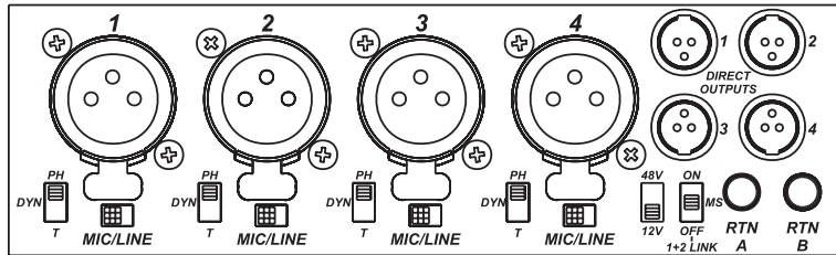
INPUT PANEL
