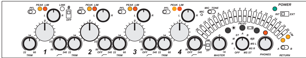
FRONT PANEL
